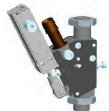
Image 3: Tiltable mouthpiece for the feeding of very short screws.
